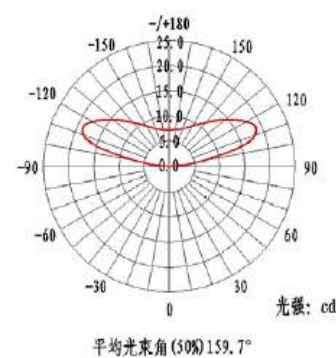
Light Distribution
